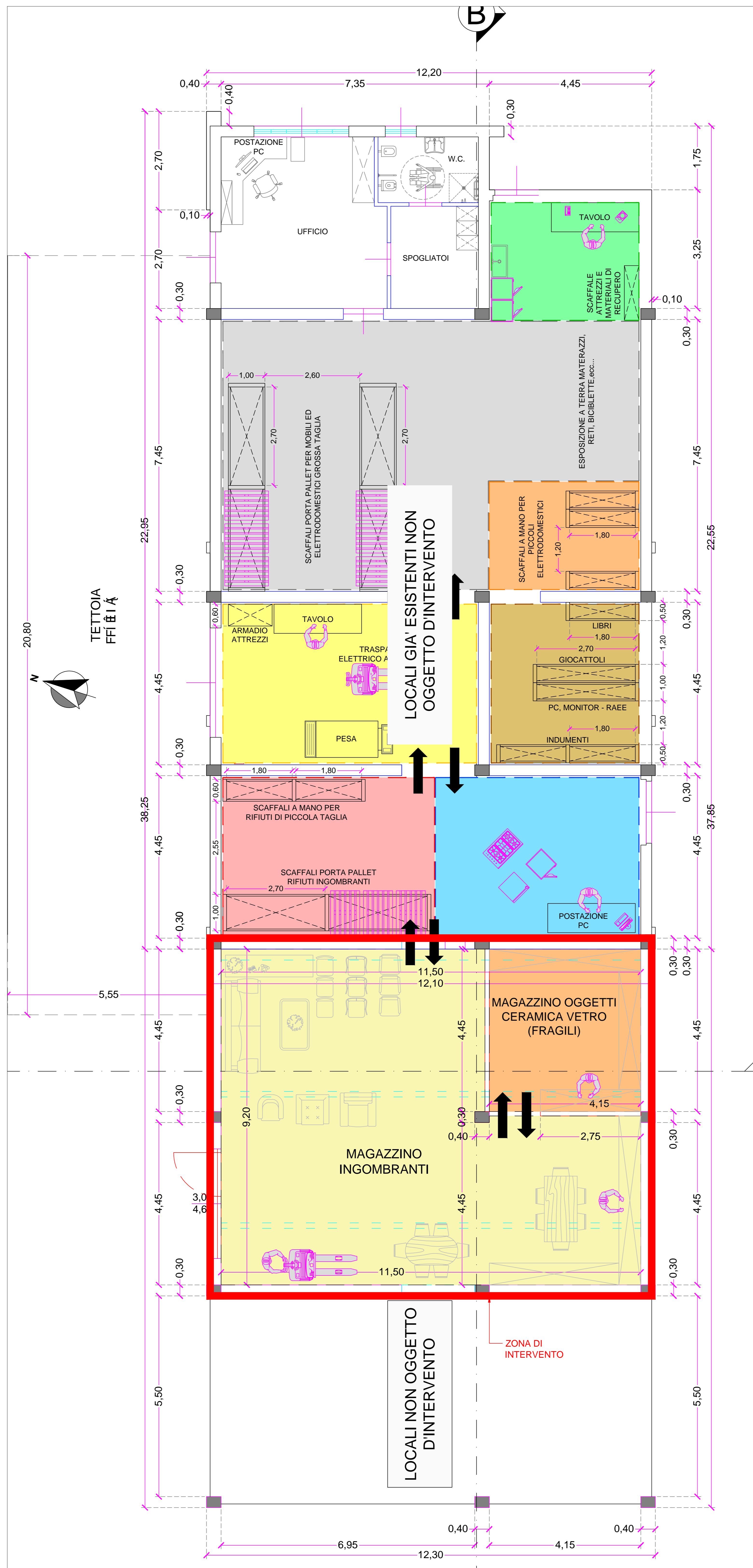
LAYOUT AREE INTERNE scala 1:50
